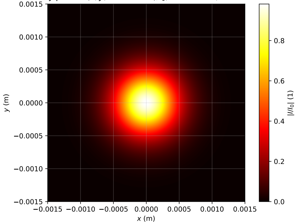
Intensity profile I(x, y, z = 1.035m)/I_0 , \text{Pin}=0.4\text{Pcr} , artificial time
